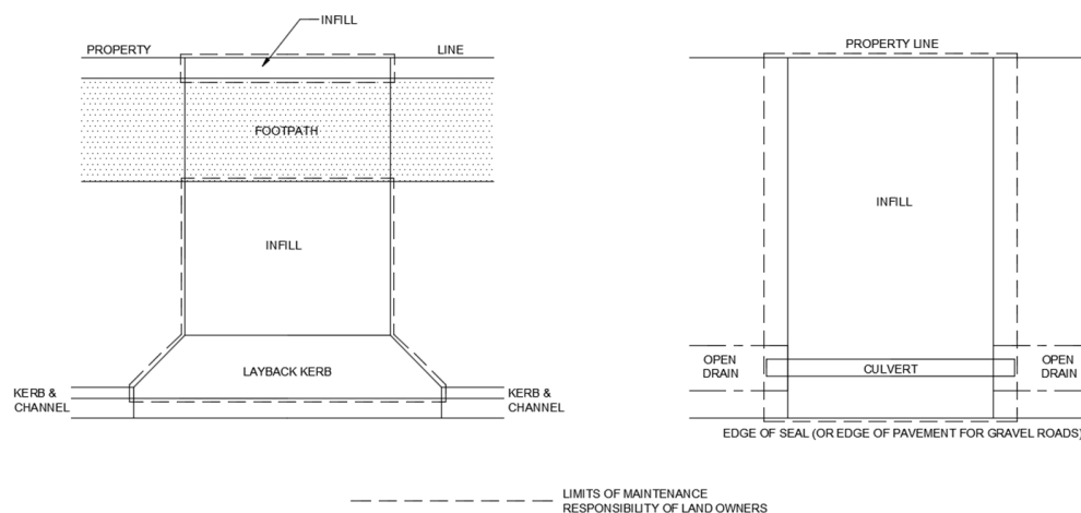
Figure 2.10.1 Limits of Maintenance Responsibility for Driveway Access
