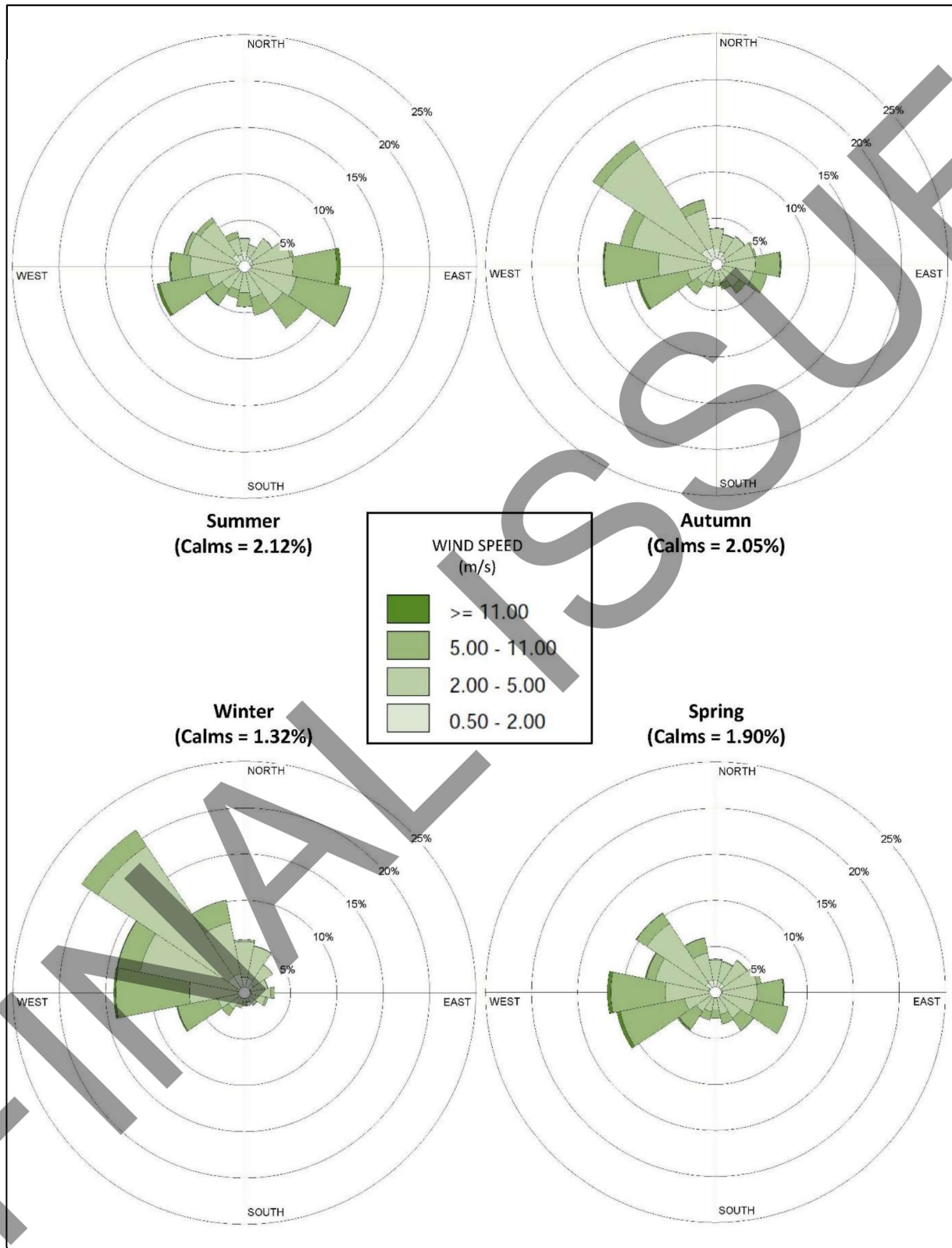
Figure 5 Seasonal wind roses based on 5-year data from BOM station number: 085279
