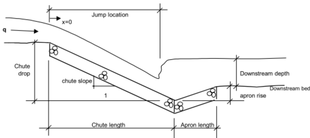
Figure 6-2 Schematic of a typical rock chute (Source: Keller (2003)).
