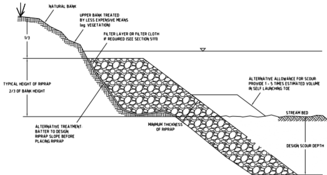
Figure 6-4 A typical rock beaching arrangement (Source: Department of Sustainability and Environment (2007)).
